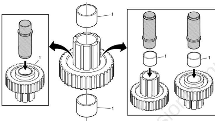
Front Output Shaft Drive Sprocket Bushing Replacement
